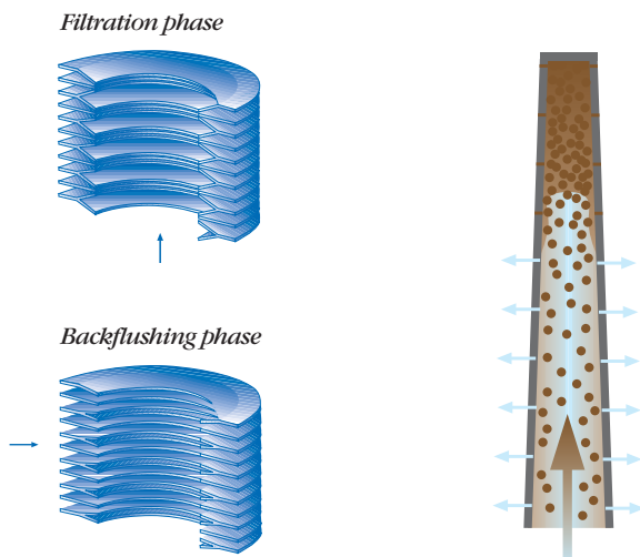
5 Expanding Disc Element
