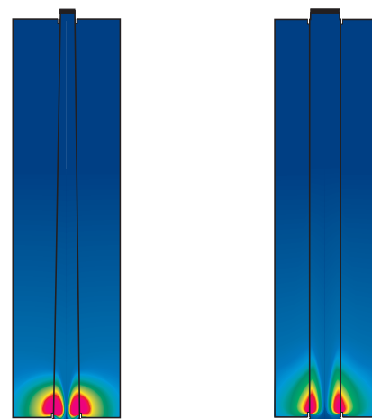
6 Conical Element
